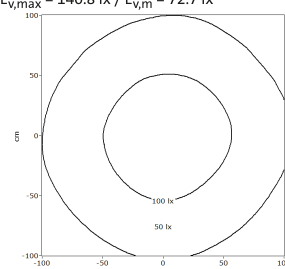
Isolux diagrams 150 cm
