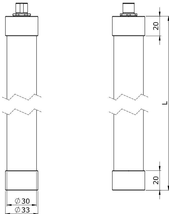
M12 Stecker 4pol M12 plug 4pol
