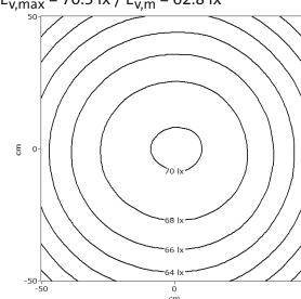
Isolux diagrams 200 cm
